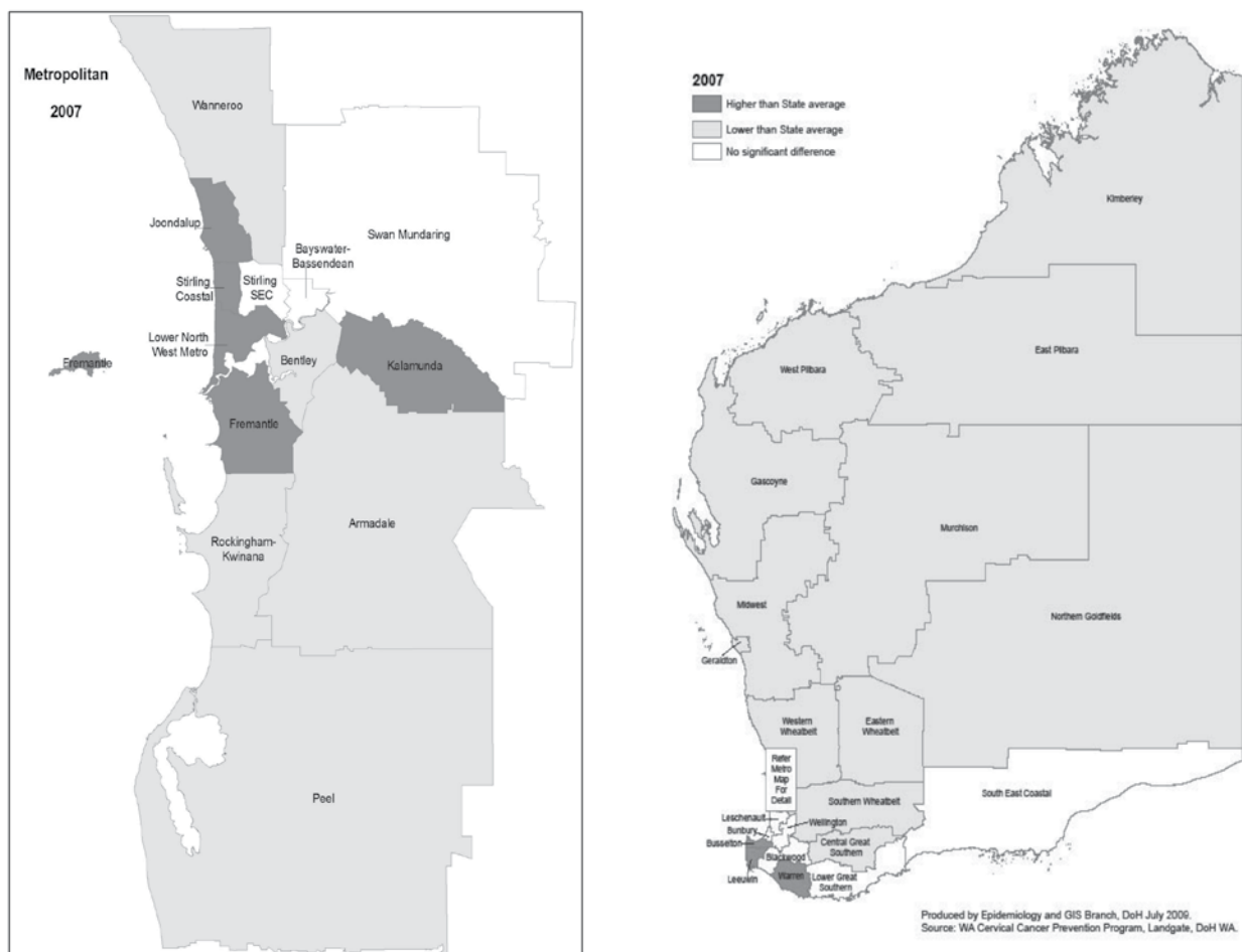
Figure 4.3 Geographical view of cervical screening participation by Health District for WA 2006-07
