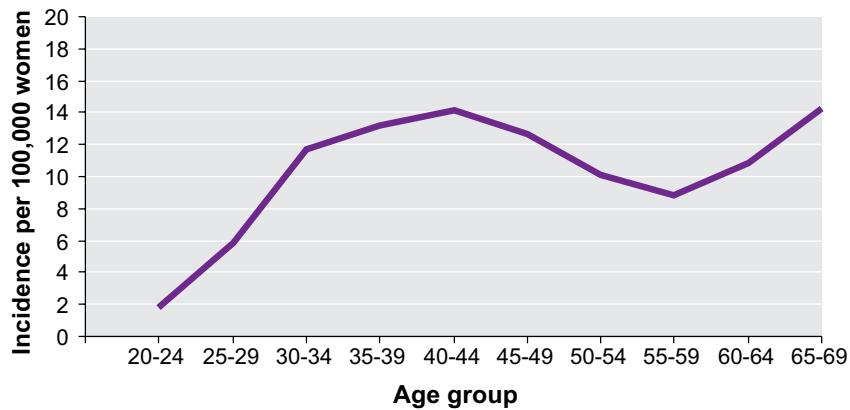
Figure 3.4 Age-specific incidence rates of cervical cancer in women aged 20-69 years WA 1997-2007
