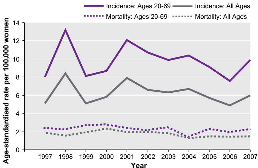
Figure 3.1 Age-standardised cervical cancer incidence and mortality rates WA 1997-2007
