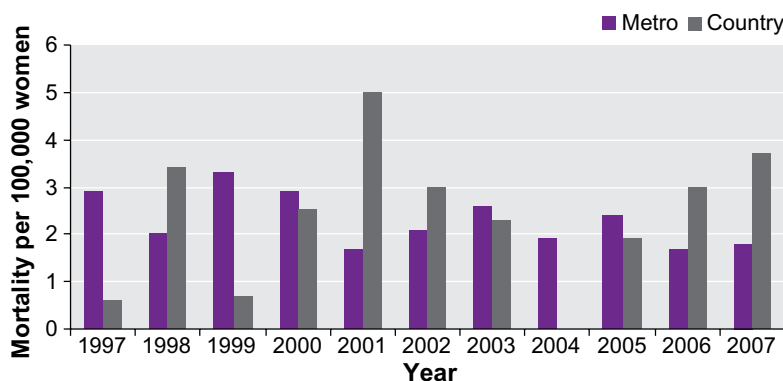
Figure 3.3 Age-standardised mortality rates from cervical cancer in women aged 20-69 years (metropolitan and country areas of WA) 1997-2007
