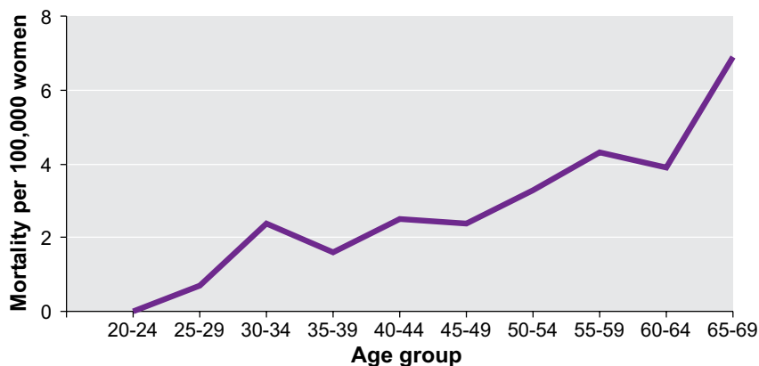
Figure 3.5 Age-specific mortality rates from cervical cancer in women aged 20-69 years WA 1997-2007
