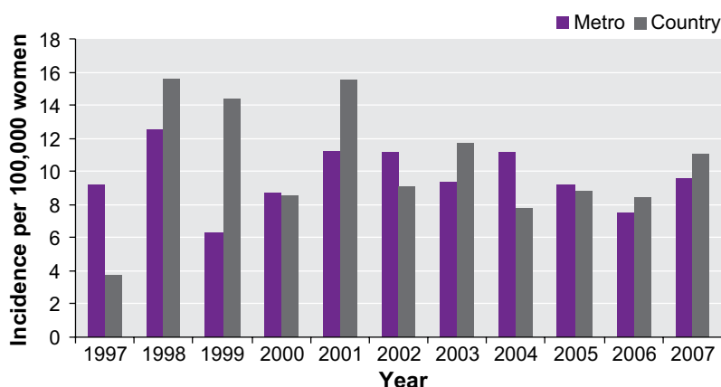
Figure 3.2 Age-standardised incidence rates of cervical cancer in women aged 20-69 years (metropolitan and country areas of WA) 1997-2007
