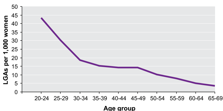
Figure 6.1 Age-specific low-grade abnormality rates in women aged 20-69 years WA 2007
