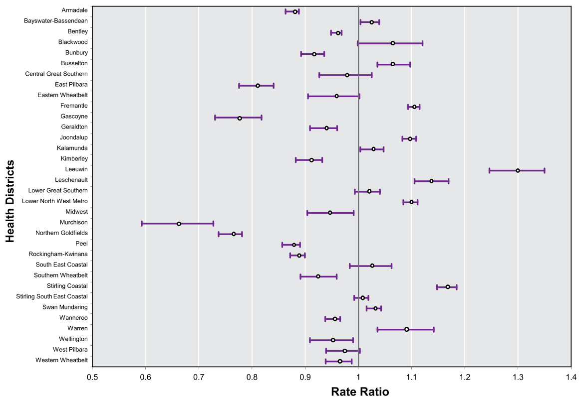
Figure 4.2 Rate ratios of cervical screening participation by Health District for WA 2006-07
