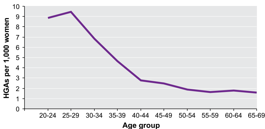
Figure 6.2 Age-specific high-grade abnormality rates in women aged 20-69 years WA 2007
