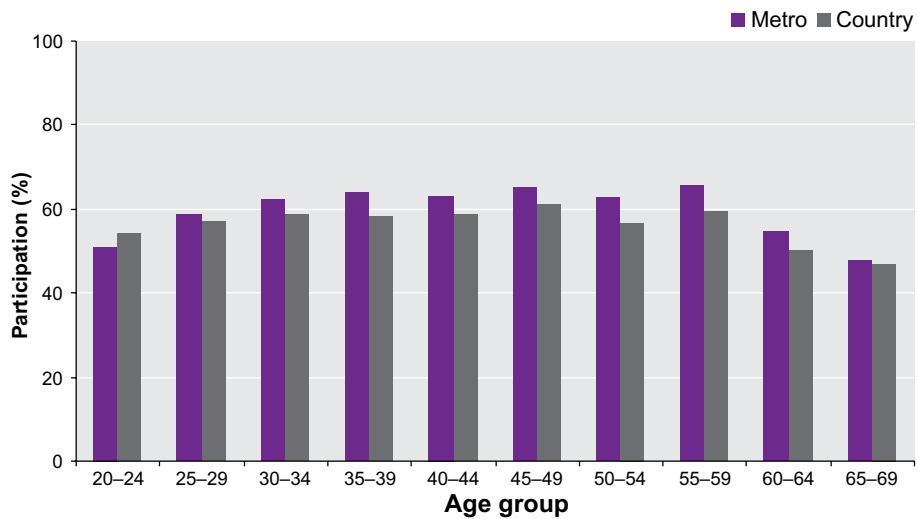
Figure 4.1 Estimated percentage of women by age group with an intact uterus who had at least one Pap smear for the two-year period 2006-2007: comparison of the Perth metropolitan area with country WA
