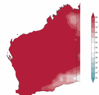
Chance of exceeding the median minimum temperature for October to December 2019
