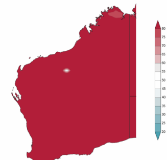
Chance of exceeding the median maximum temperature for October to December 2019
