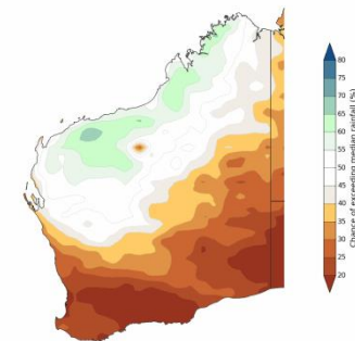
Chance of exceeding the median rainfall for October to December 2019
